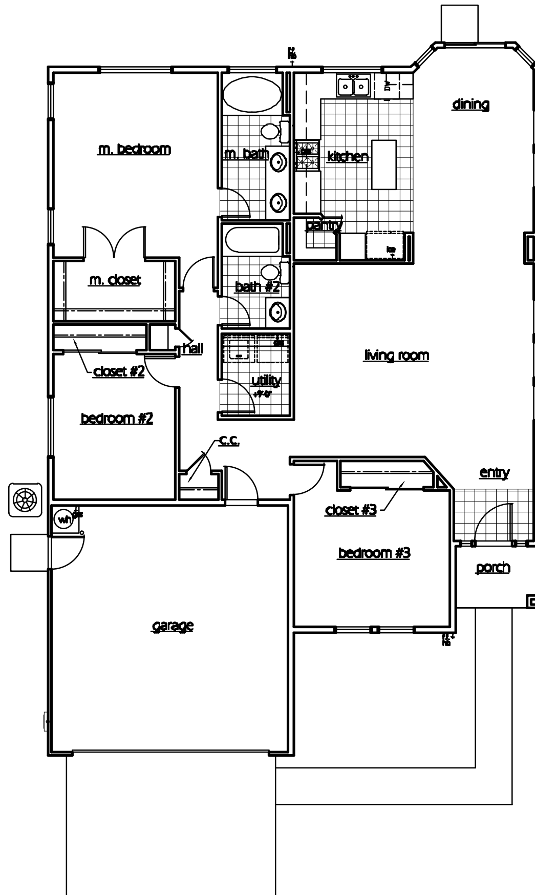
main level floor plan
